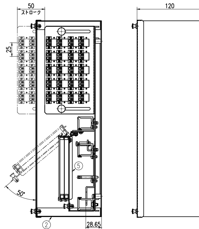
SECTION AA
